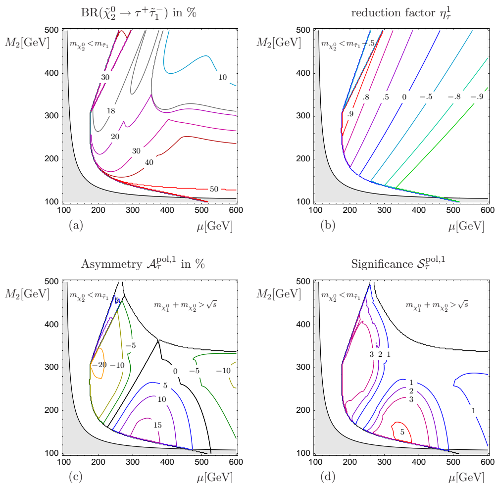
Figure 10: Neutralino production \mu^+\mu^- \rightarrow \tilde{\chi}_1^0\tilde{\chi}_2^0 and decay into a tau \tilde{\chi}_2^0 \rightarrow \tau\tilde{\tau}_1 , at \sqrt{s} = (M_{H_2} + M_{H_3})/2 with longitudinally polarized beams \mathcal{P}_- = \mathcal{P}_+ = \pm 0.3 . Contour lines in the \mu - M_2 plane for (a) the branching ratio \text{BR}(\tilde{\chi}_2^0 \rightarrow \tau^+\tilde{\tau}_1^-) , (b) the factor \eta_\tau^1 (2.32), (c) the CP-even polarization asymmetry \mathcal{A}_\tau^{\text{pol},1} , eq. (3.8), and (d) the significance \mathcal{S}_\tau^{\text{pol},1} , eq. (H.3), with the effective luminosity \mathcal{L}_{\text{eff}} = 1 \text{ fb}^{-1} , for the SUSY parameters as given in table 1. The shaded area is excluded by requiring m_{\tilde{\chi}_1^\pm} > 103 \text{ GeV} . The cross section \sigma(\mu^+\mu^- \rightarrow \tilde{\chi}_1^0\tilde{\chi}_2^0) is shown in figure 8.
